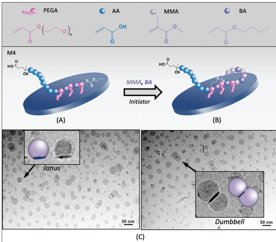
Fig. 3 Schematic representation of Laponite® platelets (A) with the adsorbed macroRAFT agent PAA 40 - b -P(PEGA 6 -co-BA 4 )-TTC (M4) and (B) during the synthesis of P(MMA-co-BA)/Laponite® nanocomposite latexes by RAFT-mediated surfactant-free emulsion polymerization using M4. (C) The cryo-TEM images of hybrid particles obtained by the copolymerization of MMA : BA 80 : 20, at 80 °C, in the presence of 2.2 mM of M4 and 5 g L -1 of Laponite® at pH 7.5 (R4B).
