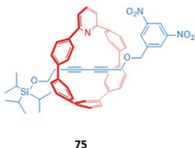
Fig. 48 Fluoride-selective self-immolating rotaxanes.
