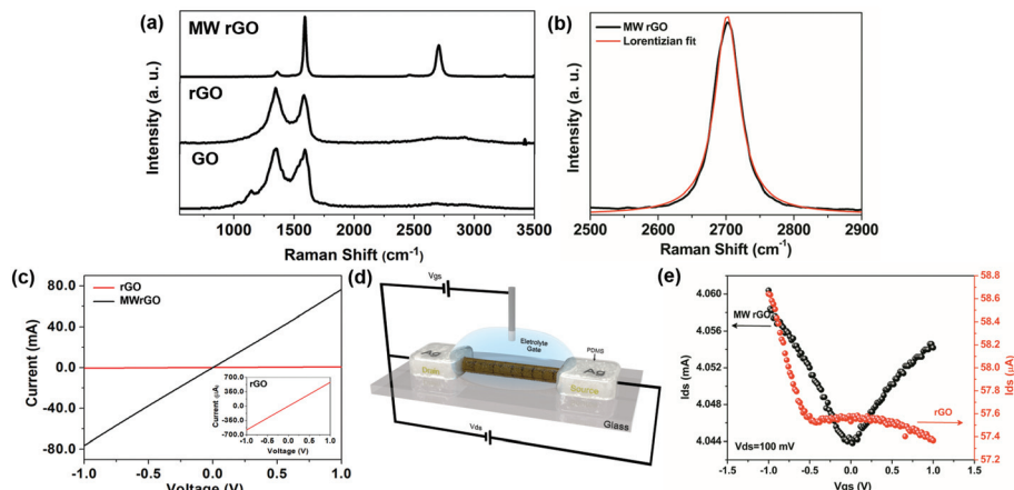
Fig. 3 (a) Representative Raman spectra for the GO, rGO and MW rGO microfibers. (b) 2D band of MW-rGO with its respective Lorentzian fit, with a FWHM of 44.01 \pm 6.62\text{ cm}^{-1} . (c) Current vs. voltage curve for the rGO and MW rGO microfibers. (d) Schematic representation of the ionic liquid gate FET based on the graphene derivative microfibers. (e) Transfer characteristics, I_{ds} vs. V_{gs} , for a V_{ds} of 100 mV in 1\text{ mol L}^{-1} of sodium fluoride aqueous solution, for the rGO and MW rGO used as a channel material in the FETs.
