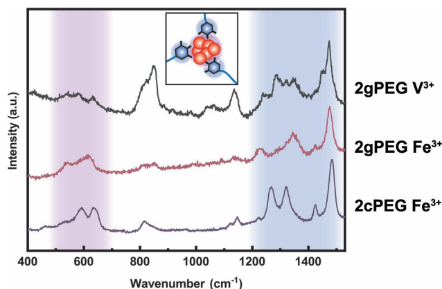
Fig. 5 Raman characterization of 2gPEG hydrogels. Resonance Raman spectra of 2gPEG crosslinked with V^{3+} and Fe^{3+} , and 2cPEG crosslinked with Fe^{3+} . The peaks between 500 and 680 cm^{-1} are attributed to the catechol- Fe^{3+} coordination or pyrogallol- Fe^{3+} coordination, while the peaks between 1230 and 1500 cm^{-1} are due to the carbon ring vibration.
