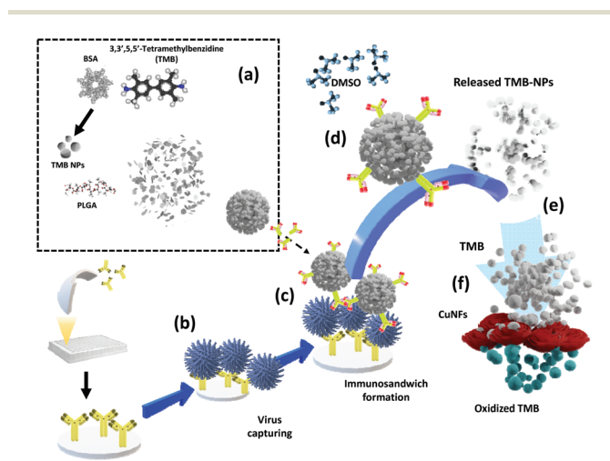
Scheme 1 The schematic illustration of the TMB-NPs@PLGA-based signal amplification platform. (a) The preparation of TMB-NPs@PLGA; (b) viruses are captured by the capture probe; (c) immunocomplex sandwich nanoconjugate with TMB-NPs@PLGA in the presence of virus; (d) addition of DMSO and the dissolution of the PLGA nanovesicle; (e) the release of TMB-NPs due to the dissolution of TMB-NPs by DMSO, and (f) the catalytic oxidation of TMB by CuNFs/ \text{H}_2\text{O}_2 for colorimetric detection.
