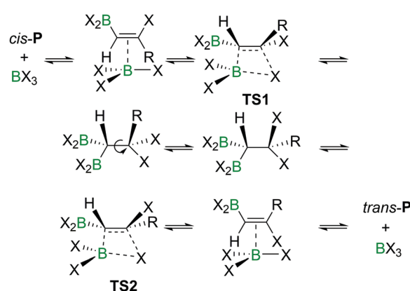
Scheme 7 Possible mechanism for stereoconversion mediated by BX_3 .
