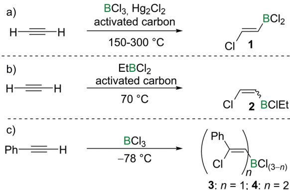
Scheme 1 Chloroboration of acetylene/phenylacetylene under various conditions.
