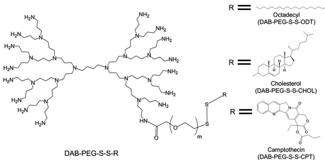
Fig. 5 Chemical structure of an amphiphilic, surface-modified, disulfide-linked octadecyl chain-bearing/cholesterol-bearing/camptothecin-bearing PEGylated generation 3-diaminobutyric polypropyleneimine (PPI or DAB) dendrimer (DAB-PEG-S-S-ODT/DAB-PEG-S-S-CHOL/DAB-PEG-S-S-CPT respectively), where m = 45 .
