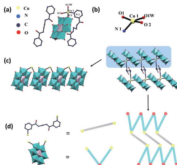
Fig. 7 (a) The single molecule, (b) partial enlarged drawing of the Cu coordination site, (c) packing model, and (d) the ball-stick model of the Anderson-type polyoxomolybdate H\{Cu_{L_{0.5}^1}[CrMo_6(OH)_6O_{18}](H_2O)\} \cdot 0.5 L^1 ( L^1 = N,N' -bis(3-pyridinecarboxamide)-1,2-ethane). 95
