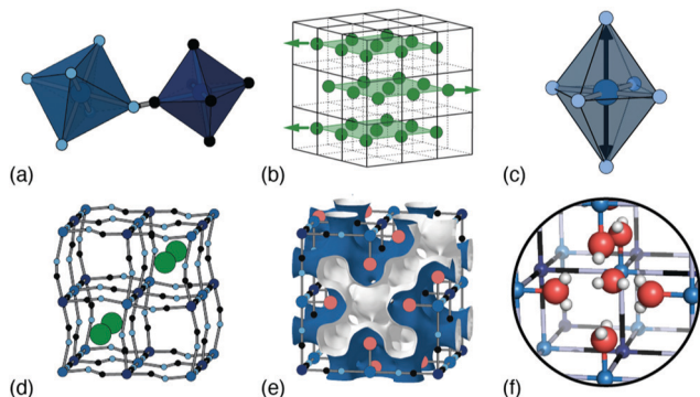
Fig. 1 Common types of structural complexity in PBAs: (a) octahedral tilts, (b) correlated 'slides' of A-site cations, (c) Jahn–Teller distortions, (d) A-site occupancy (dis)order, (e) hexacyanomethylate vacancies and the resulting connected pore-network structure, and (f) framework hydration.
