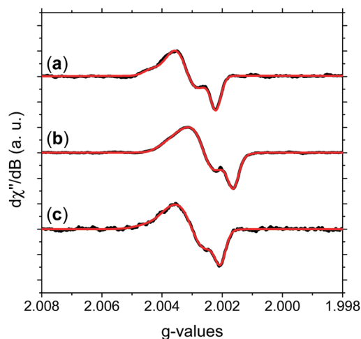
Fig. 3 Experimental HFEPD derivative absorption spectra (black line) and their fitting (red line) for (a) NFMel, (b) NFMel-P and (c) SMel at 0.1 mW microwave power. Fitting parameters are displayed in Table 1.
