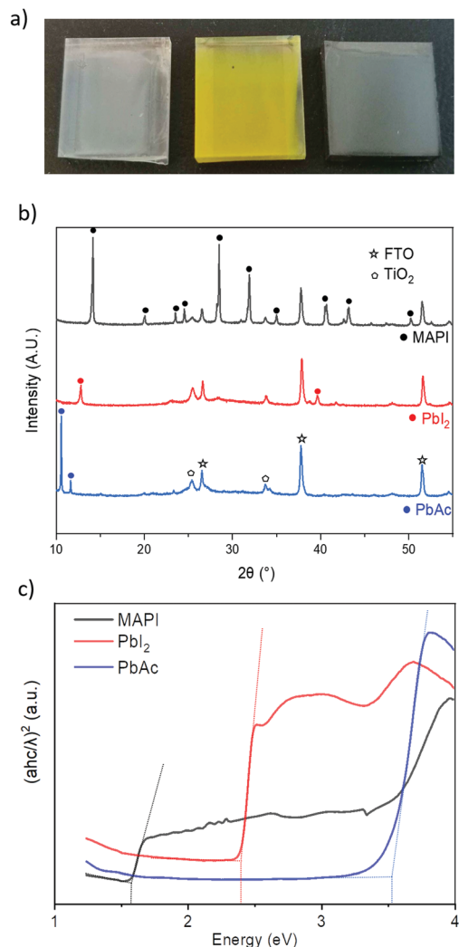
Fig. 3 (a) Photographs of three films removed at different stages of the AACVD deposition (substrate size 12 mm × 12 mm). Left: Film after first step. Centre: Film halfway through MAI aerosol exposure. Right: Completed MAPI film (b) XRD patterns correspond to initial PbAc 2 film, PbI 2 intermediary and final MAPI film (c) Tauc plots of the three films calculated from absorption data.
