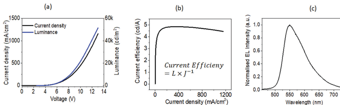
Fig. 3 Characteristics of OLEDs: (a) current density and luminance as a function of voltage, (b) current efficiency as a function of current density, (c) EL spectrum of an OLED. All graphs are taken from our work from OLEDs (structure: glass/ITO/PEDOT:PSS/Super Yellow ((poly(para-phenylene vinylene)copolymer))/Ca/Al).
