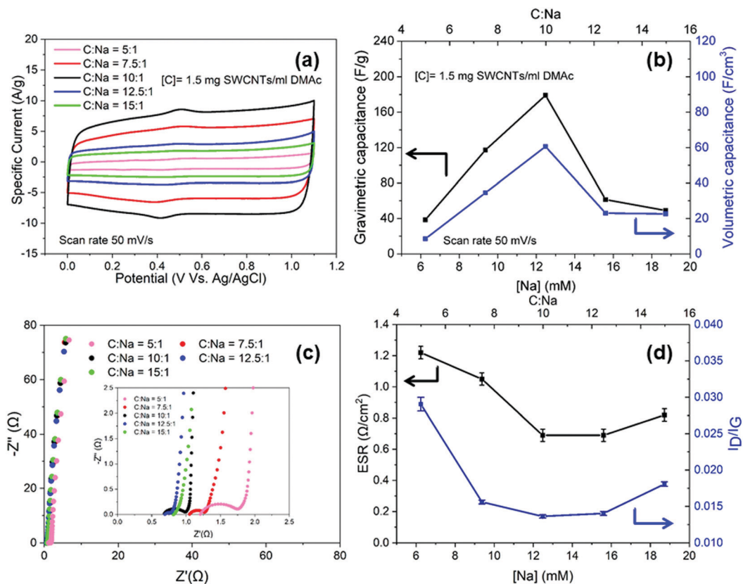
Fig. 2 Half-cell electrochemical performance, in 1 M H 2 SO 4 , of nanotubide buckypapers prepared from solutions at a given sodium concentration, or equivalent C : Na ratio: (a) CV curves at 50 mV s -1 ; (b) gravimetric and volumetric capacitance of (a) normalised to the mass and volume of active electrode; (c) Nyquist plots and (d) ESR and the I D to I G ratio derived from Raman spectra.
