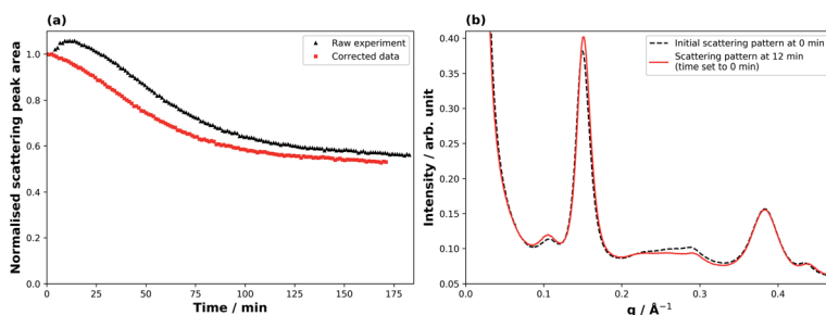
Fig. 2 Illustration of data correction (film thickness: 73 \pm 2 \mu\text{m} ). (a) Scattering peak area vs. time exposed to ozone; both raw and corrected data are plotted. (b) SAXS patterns of the sample at the beginning of the experiment (black dashed line) and at the time (after 12 min) at which the peak scattering area was measured, which was defined as t = 0 for the decay of the lamellar phase (red solid line).
