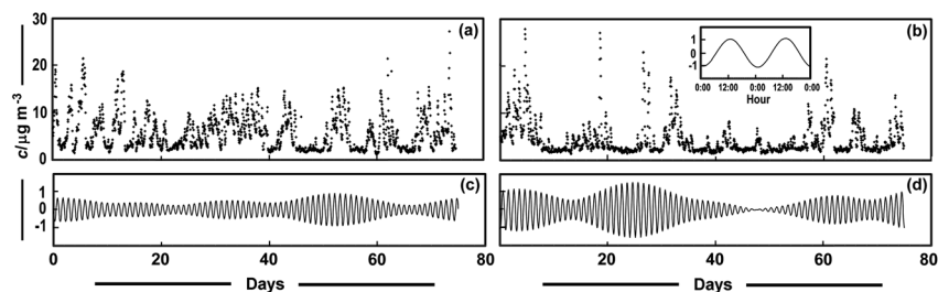
Fig. 4 Daily average \text{SO}_2 concentrations over 75 days starting on 24th January of 2019 (a) and 2020 (b), with concentration signals with a daily periodicity ( i.e. 23–25 h) displayed for both 2019 (c) and 2020 (d). The inset of (b) shows the concentration signal with a daily periodicity for 24th and 25th January.
