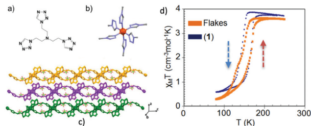
Fig. 8 (a) The tris-tetrazole ligand ( \text{L}_1 ); (b) the representation of the \text{Fe}_6 chromophore in [\text{Fe}(\text{L}_1)_2](\text{ClO}_4) where \text{Fe}(\text{II}) is shown as a red sphere; (c) packing of the 2D sheets along the b -axis; (d) temperature dependence of the susceptibility data, in the form of \chi_M T , of the exfoliated flakes (orange) and the crystals (blue) confirming the spin transition phenomenon. Adapted from ref. 50 with permission from the American Chemical Society, copyright 2018.
