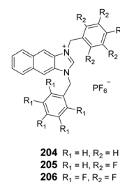
Fig. 29 Structure of compounds 204–206 .
