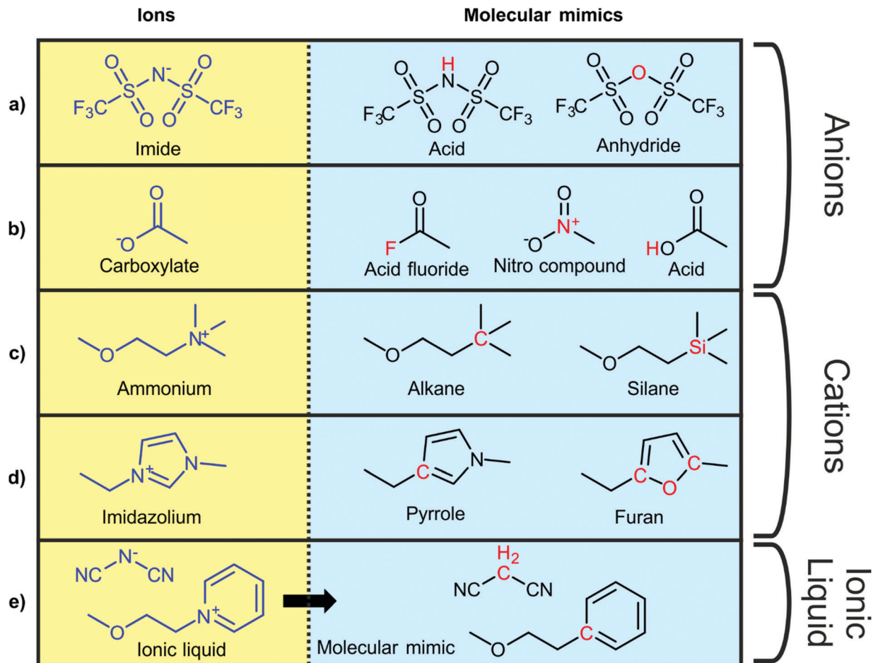
Fig. 3 Typical ionic liquid ions (left) and their targeted modifications to yield molecular mimics (right).
