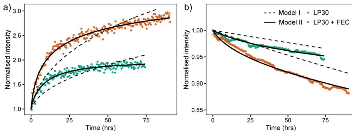
Fig. 9 The intensity changes of the ^7\text{Li} NMR spectra (points) and the model fit results for Model I (dashed lines) and Model II (black lines) for (a) the lithium metal and (b) the lithium ions, in the two electrolytes LP30 (green) and LP30 + FEC (orange).
