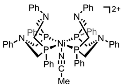
Scheme 1 Structure of [\text{Ni}(\text{P}^{\text{Ph}}_2\text{N}^{\text{Ph}}_2)_2(\text{CH}_3\text{CN})]^{2+} .
