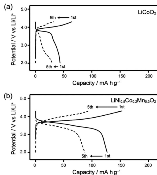
Fig. 8 Charge–discharge curves of Li half-cells composed of LC electrolyte 1/LiTFSI and various transition metal positive electrodes recorded at 80 ^{\circ}\text{C} ; (a) \text{LiCoO}_2 and (b) \text{LiNi}_{0.5}\text{Co}_{0.2}\text{Mn}_{0.3}\text{O}_2 .
