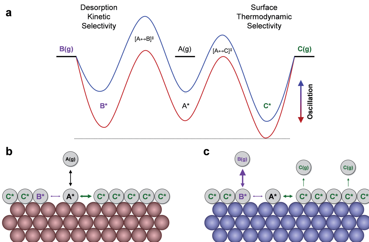
Fig. 4 Mechanisms of dynamic selectivity to products in parallel chemistry. (a) Oscillation of surface binding energies of A*, B*, and C* between strong (red) and weak (blue) enthalpy of adsorption occurs through two transition states. Two general behaviors can produce high selectivity to specific products: weak surface binding permitting reaction surface resonance to product B(g), or strong surface binding that leads to a C* dominated surface. (b) The surface filling state. (c) The surface turnover state. Chemical dynamic parameters: \gamma_{B/A} = 1.3 , \gamma_{C/A} = 0.6 , and \delta_{B-A} = 0.6 eV, \delta_{C-A} = 1.5 eV, U_l = -0.5 eV, \Delta U = 0.4 eV.
