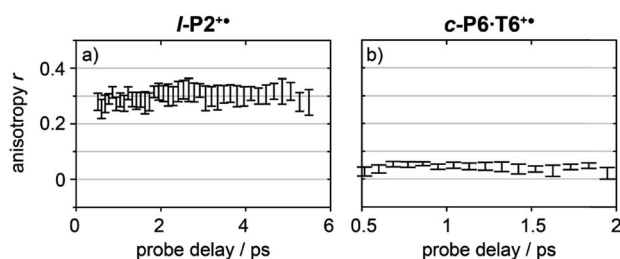
Fig. 6 Average anisotropy of all analyzed signals (greyed areas in Fig. 5a and b) of \text{I-P2}^{+\bullet} (a) and \text{c-P6}\cdot\text{T6}^{+\bullet} (b) pumped both at 2100\text{ cm}^{-1} and 3250/2500\text{ cm}^{-1} as a function of probe time delay.
