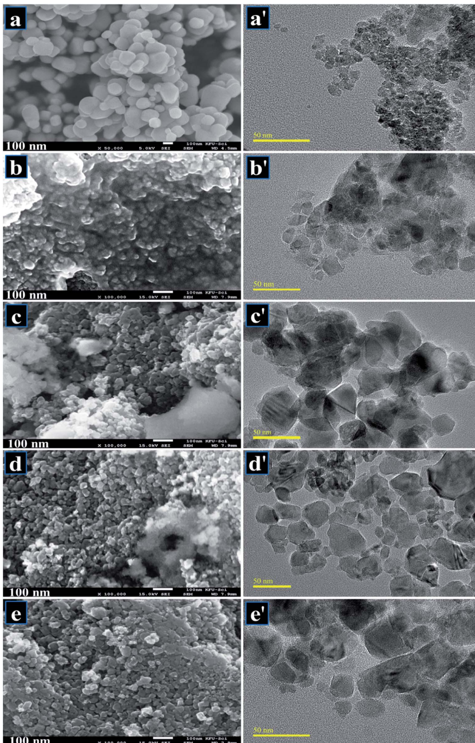
Fig. 7 (a–e) FESEM images of 0 : 1, 0.02 : 1, 0.04 : 1, 0.06 : 1, and 0.08 : 1 samples, respectively (a'–e') corresponding HR-TEM micrographs of TiO 2 and 0 : 0.02 : 1, 0.04 : 1, 0.06 : 1, and 0.08 : 1 samples, respectively.
