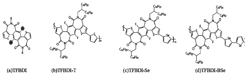
Fig. 7 Some monomers of fluorinated dithienylbenzodioxoles (a–d).
