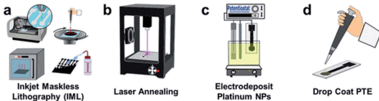
Fig. 7 Schematic representation of the fabrication process of PtNP-IML-PGE biosensor. First graphene is patterned by IML (a) followed by annealing with laser (b) electrodeposition of Pt NPs (c) and drop-coating of PTE ink (d). Reprinted with permission from ref. 66. Copyright (2018) American Chemical Society.
