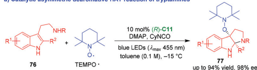
b) Application in total synthesis of (–)-verrupyrrroloindoline
