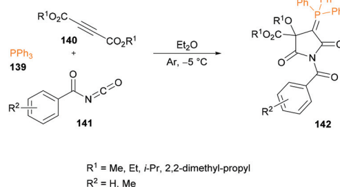
Scheme 32 Three-component synthesis of highly functionalized triphenylphosphoranyliden succinimides.
