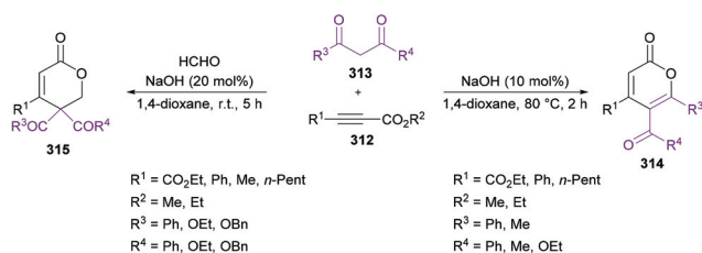
Scheme 79 Synthesis of polysubstituted 2 H -pyran-2-ones from alkyne and activated methylenes.
