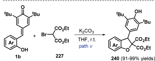
Scheme 52 [4 + 1] annulation toward 2,3-dihydrobenzofurans.
