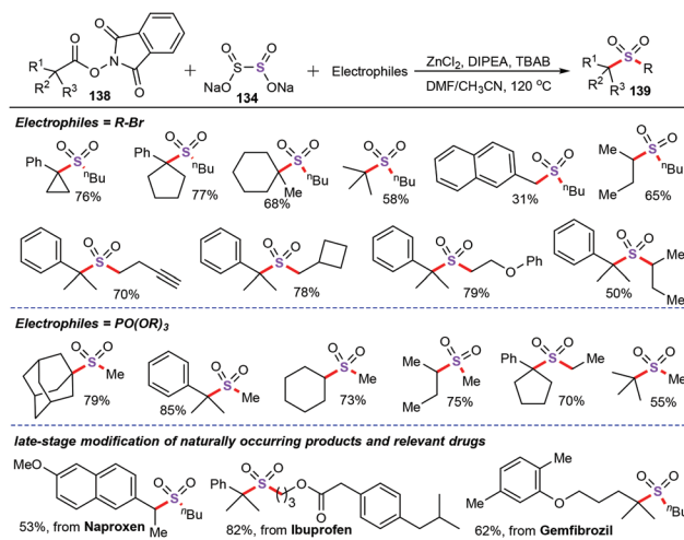
Scheme 51 Sodium dithionite-mediated decarboxylative sulfonylation.
