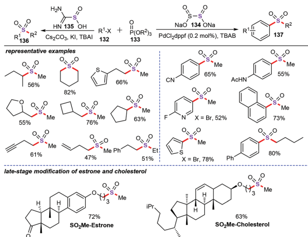
Scheme 50 General sulfone construction via SO 2 surrogate control.
