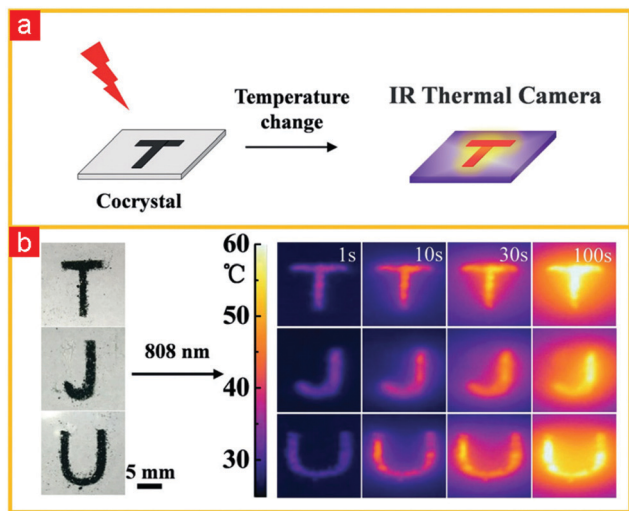
Fig. 5 (a) Diagram of photothermal imaging process. (b) IR camera images of cocystal-patterned letters TJU. 69 (Reprinted with permission from Wiley-VCH. Copyright 2018.)
