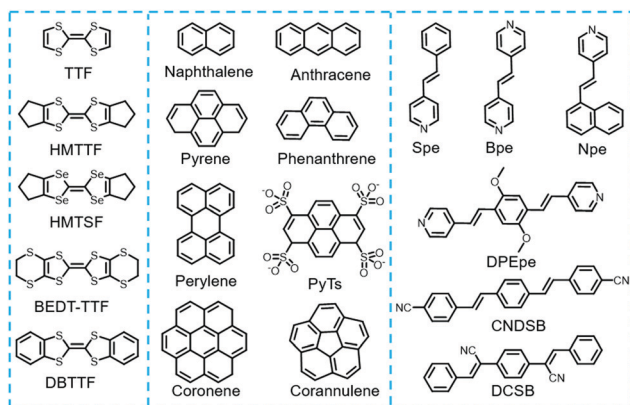
Fig. 6 Molecular structures of typical donors of cocystals.
