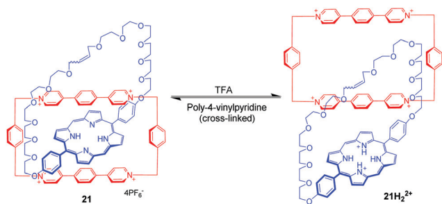
Fig. 21 pH-Controllable [2]catenane 21 .
