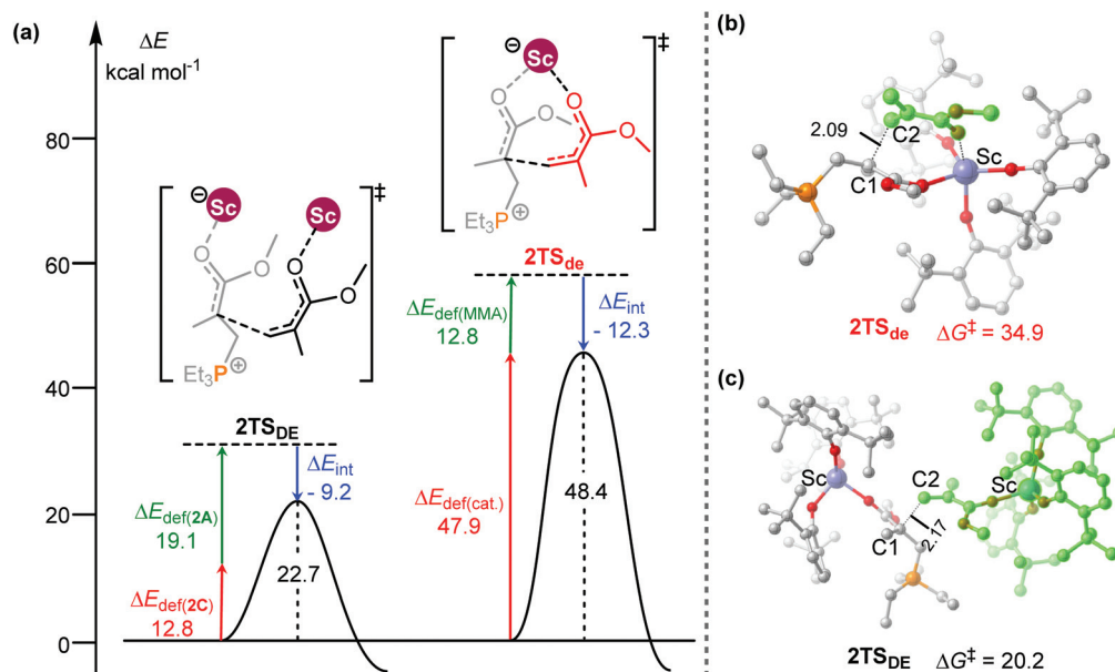
Fig. 3 (a) Distortion/interaction analyses ( \text{kcal mol}^{-1} ) and geometric parameters (distances in \text{\AA} ) of (b) 2\text{TSD}_{de} and (c) 2\text{TSD}_E .
