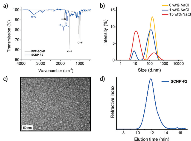
Fig. 3 Characterization of functionalization of PFP-SCNP with 1-aminoglycerol ( SCNP-F2 ) (a) overlapped FT-IR spectra of PFP-SCNP and SCNP-F2 ; (b) DLS spectra at different salt concentrations in water; (c) TEM image; (d) SEC trace.
