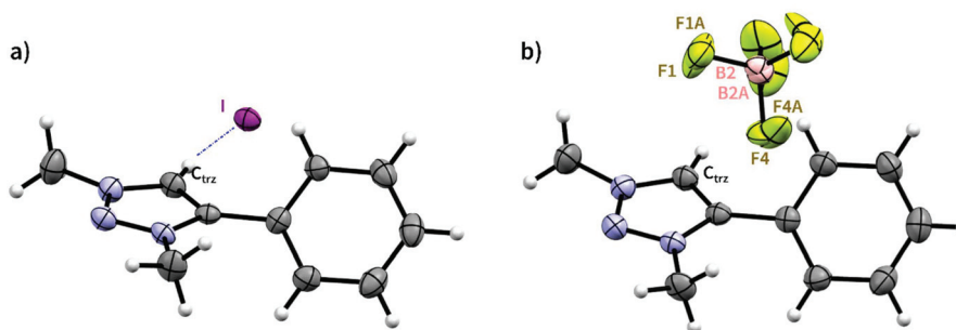
Fig. 1 (a) Molecular structure of triazolium salt 1 , determined by single crystal X-ray diffraction analysis. Selected bond lengths (Å) and angles (°): |C_{tr2} \cdots I| = 3.783(3) , |H_{tr2} \cdots I| = 2.857 , \angle C_{tr2}-H_{tr2} \cdots I = 173.69 . (b) Molecular structure of triazolium salt 1' , determined by single crystal X-ray diffraction analysis. BF_4 anion is disordered over two sites B2 (65.2%) and B2A (34.8%).
