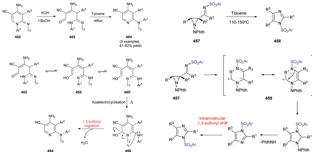
Scheme 64 Thermal rearrangement of 5-oxo-pent-3-enimides to 4-aminopyridines via 1,3-nitrogen-to-nitrogen sulfonyl migration.
