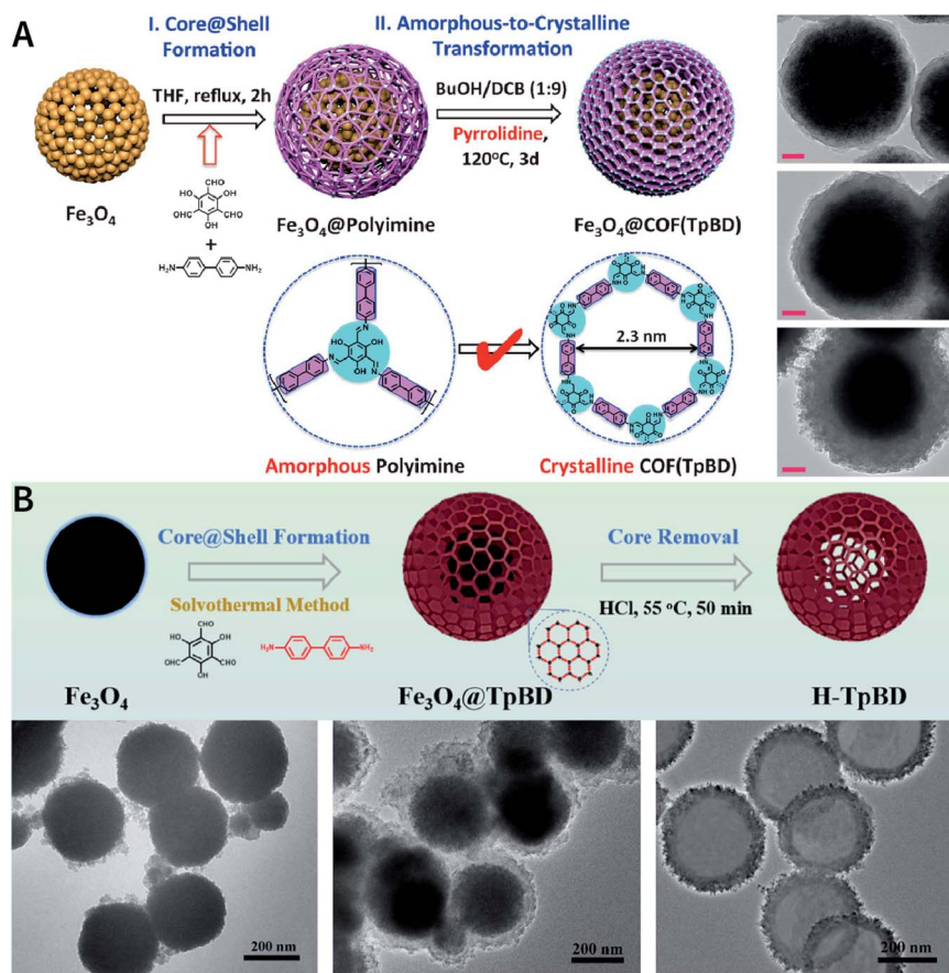
Fig. 38 (A) Preparation protocol and HRTEM images of \text{Fe}_3\text{O}_4@ COF (TpBD) with shell thicknesses of 20, 50, and 100 nm. Scale bar: 50 nm. Adapted with permission. 232 Copyright 2016, Wiley-VCH Verlag GmbH & Co. KGaA, Weinheim. (B) Synthesis protocol and HRTEM images of hollow COF nanoshells. Adapted with permission. 233 Copyright 2018, Elsevier B.V.
