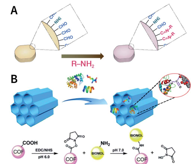
Fig. 52 (A) BDF of imine-linked COFs. (B) Grafting biomolecules on the surface of NKCOF-1 COF containing carboxyl groups via BDF. Adapted with permission. 323 Copyright 2018, Wiley-VCH Verlag GmbH & Co. KGaA, Weinheim.
