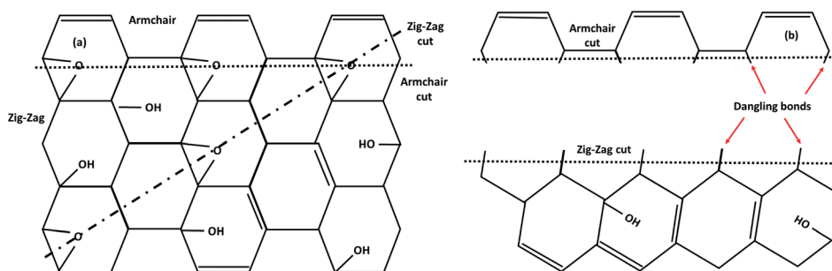
Fig. 13 (a) A pictorial representation of unzipping of graphene oxide via (b) zig-zag and/or armchair cutting.
