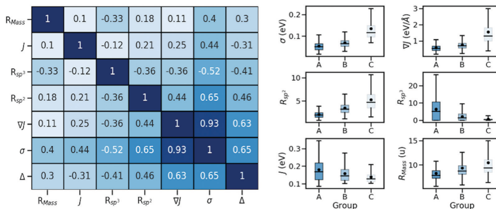
Fig. 2 (left) Spearman's rank correlation between parameters. (right) Variation range of parameters correlated with the relative dynamic disorder ( i.e. \sigma , \nabla J , R_{\text{sp}^2} , R_{\text{sp}^3} , J and R_{\text{Mass}} ) among defined categories of A, B, and C depicted on a series of "box plots". The box limits represent the first (Q1) and third quartiles (Q3), with a line and a small circle representing the median and the mean value, respectively.
