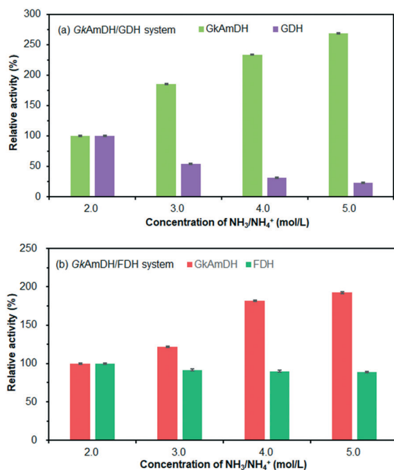
Fig. 2 The relative activity of GkAmDH and GDH in \text{NH}_3\cdot\text{H}_2\text{O}/\text{NH}_4\text{Cl} buffer (a) and GkAmDH and FDH in \text{NH}_3\cdot\text{H}_2\text{O}/\text{NH}_4\text{COOH} buffer (b). The activity of the enzymes in buffer containing 2 M \text{NH}_3/\text{NH}_4^+ was normalized as 100%.
