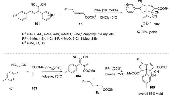
Scheme 32 Phosphine-catalysed sequential (2+3) and (3+2) annulation reactions of \gamma -substituted allenates with conjugated dienes.
