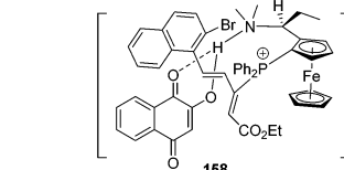
Scheme 50 Phosphine catalysed atroposelective (4+2) annulations of \delta -acetoxy allenates with 2-hydroxyquinone derivatives.
