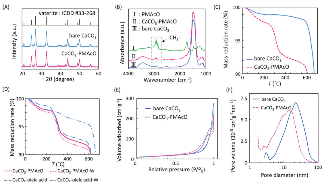
Fig. 3 Physical properties of bare CaCO 3 and CaCO 3 -PMAcO microspheres: (A) XRD spectra, (B) FT-IR spectra, (C) TG curves, (D) TG curves of CaCO 3 -PMAcO and CaCO 3 -oleic acid before and after washing; "-W" indicates samples after washing, (E) N 2 adsorption-desorption isotherms, and (F) pore size distributions.
