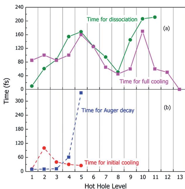
Fig. 5 (a) The times for molecule dissociation and the times for full nonadiabatic cooling of the hot hole carriers (the time to reach thermodynamic equilibrium); (b) the times for Auger decay and the times for initial cooling (the occupation of the initial ionized level increases to 2) of the hot hole carriers after one electron is ejected and a hot hole is formed on different levels of C_2H_6O_2 . The Auger decay can only occur for Level 1–5.
