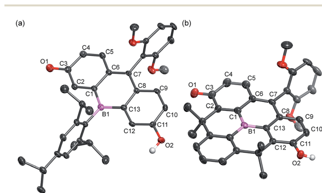
Fig. 2 Crystal structures of (a) BF2 and (b) BF3 (50% probability of thermal ellipsoids). Hydrogen atoms, except for those on the phenolic hydroxy groups, are omitted for clarity.
