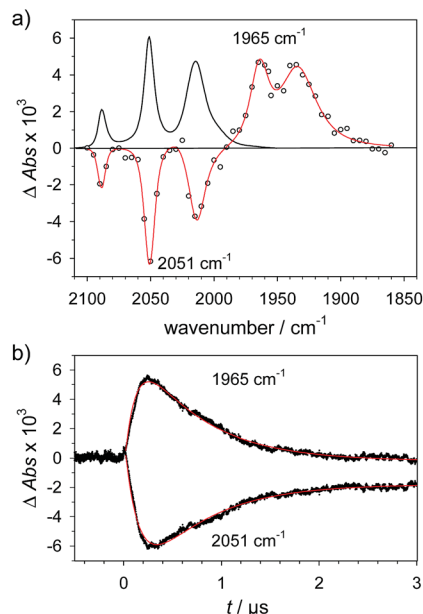
Fig. 5 (a) Transient IR spectrum 0.3 \mu s after excitation (O, \text{---} ) and normalized IR spectrum of the starting state ( \text{---} ) for formation of 1\text{H} by reduction of 1\text{H}^+ (obtained by protonation of 1 with 2.6 mM \text{Cl}_2\text{BSA} ) with flash-quench generated [\text{Ru}(\text{dmb})_3]^+ in acetonitrile. (b) Kinetic traces ( \cdots ) and fits ( \text{---} ) monitoring pseudo-first order formation of 1\text{H} ( 1965\text{ cm}^{-1} ) and bleach of 1\text{H}^+ ( 2051\text{ cm}^{-1} ) followed by pseudo-first order decay of 1\text{H} by protonation with \text{Cl}_2\text{BSA} and charge recombination with \text{TTF}^+ .
