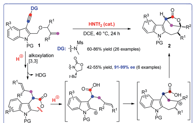
Scheme 1 Catalytic alkene carboxygenation via a C–O cleavage.
