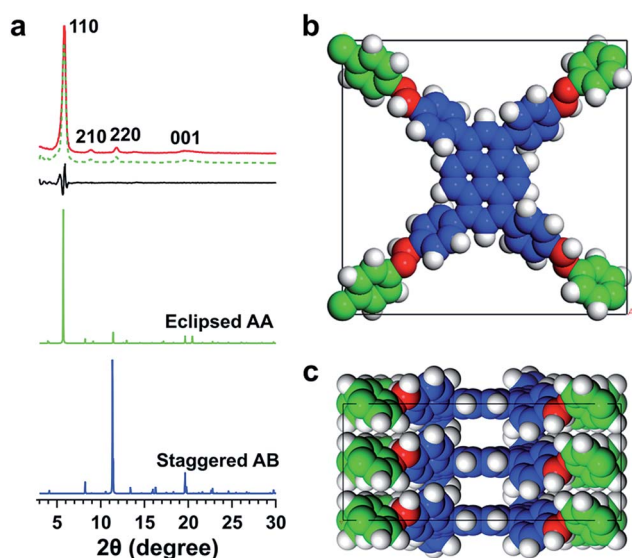
Fig. 1 (a) PXRD patterns of TFPPy-ETTA-COF (red), the Pawley refinement (dotted green) and their difference (black), eclipsed AA (green), and AB (blue) stacking modes. (b) Top and (c) side views of the unit cell.
