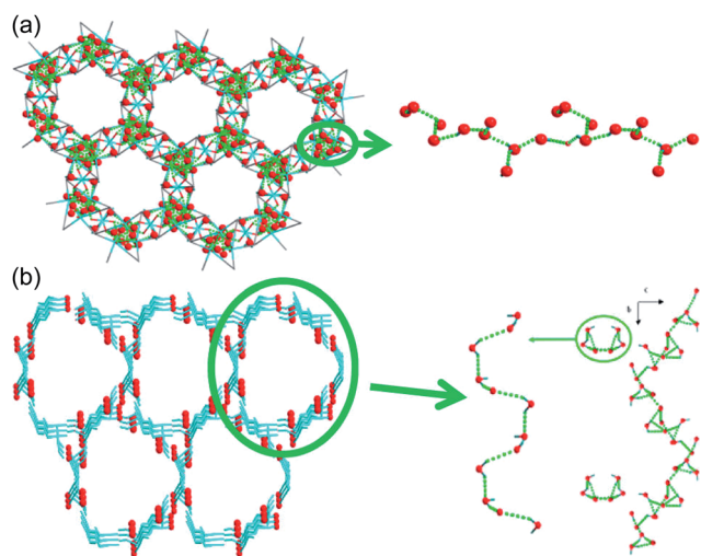
Fig. 17 1-D channels with water molecules in (a) \{[\text{Co}_3(m\text{-ClPhIDC})_2(\text{H}_2\text{O})_6] \cdot 2\text{H}_2\text{O}\}_n ( 1 ) and (b) \{[\text{Co}_3(p\text{-ClPhIDC})_3(\text{H}_2\text{O})_3] \cdot 6\text{H}_2\text{O}\}_n ( 2 ). Red spheres represent O atoms in water, and green dots present H-bonding networks. Reproduced from ref. 74 with permission from American Chemical Society, Copyright 2017.
