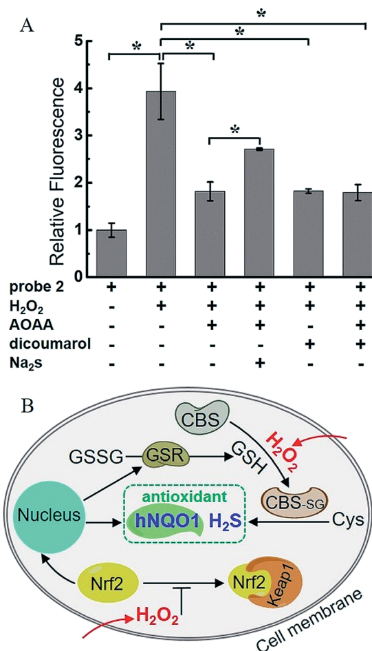
Fig. 8 (A) Relative fluorescence intensity of confocal microscopy images from H 2 O 2 -induced HeLa cells. N = 3 fields of cells, error bars are means ± s.d. * P < 0.05. (B) A proposed mechanism of the synergistic antioxidant effect of H 2 S and hNQO1 under oxidative stress.
