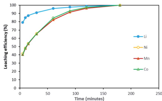
Fig. 3 Leaching kinetics of NMC 811 in 4 mol L -1 HCl at S/L = 20 g L -1 and 25 °C.
