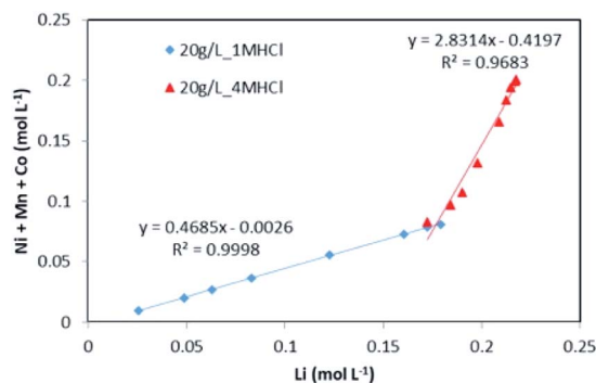
Fig. 5 Stoichiometry between the sum of Ni, Mn, Co concentration and Li concentration in leachate at S/L = 20 g L -1 during NMC 811 dissolution by 1 mol L -1 (blue diamonds) and 4 mol L -1 HCl (red triangles) at 25 °C.
