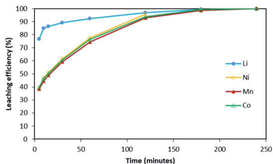
Fig. 2 Leaching kinetics of NMC 811 in 4 mol L -1 HCl at S/L = 2 g L -1 and 25 °C.
