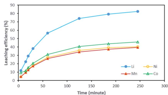
Fig. 4 Leaching kinetics of NMC 811 in 1 mol L -1 HCl at S/L = 20 g L -1 and 25 °C.
